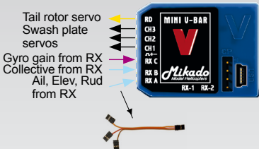
Diagram for use with standard receivers.
