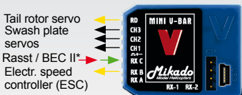
Diagram for use with Rasst, S-Bus, Jeti and other single-line receivers.
